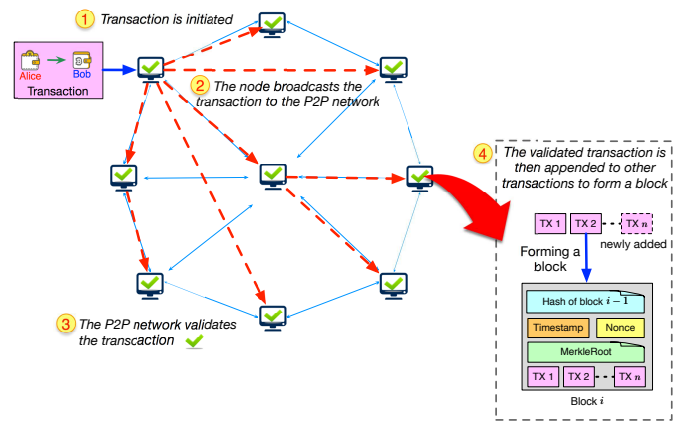
Fig. 3. Working flow of blockchains
